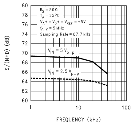
Unipolar Signal-to-Noise + Distortion Ratio vs. Input Frequency
