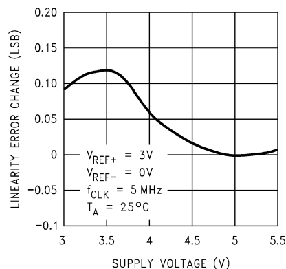
Linearity Error Change vs. Supply Voltage
