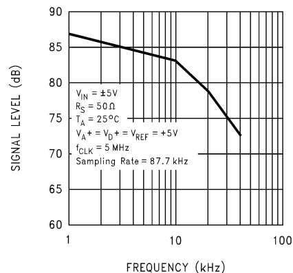
Bipolar Spurious Free Dynamic Range
