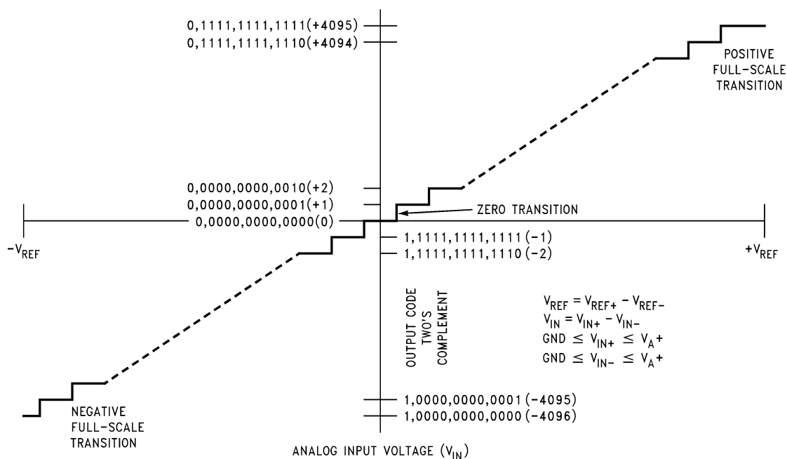
FIGURE 5. Transfer Characteristic
