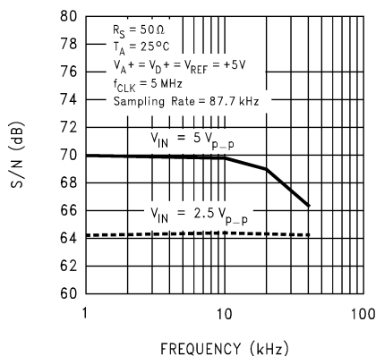
Unipolar Signal-to-Noise Ratio vs. Input Frequency
